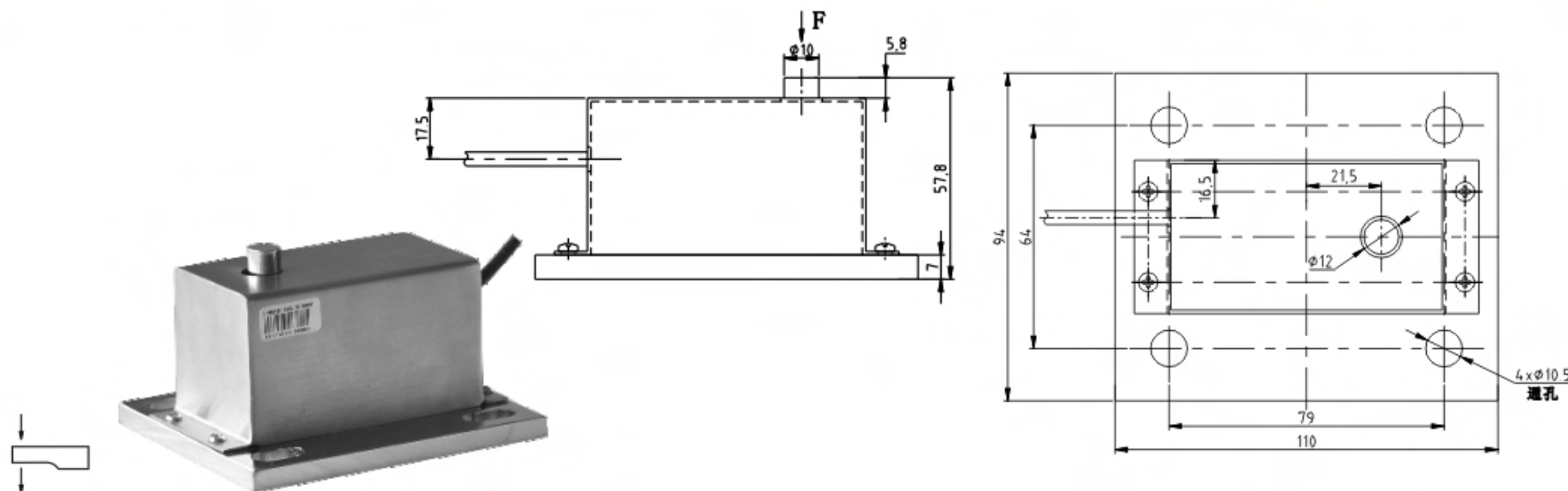
皮带秤 Belt scale
